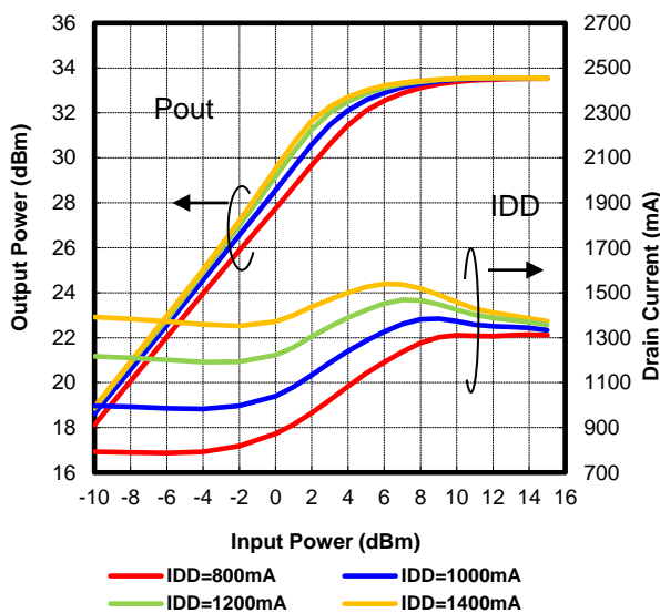
VDD=6V, Freq.=13.5GHz
