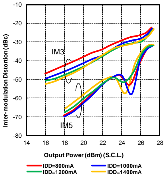
VDD=6V, Freq.=15.4GHz
