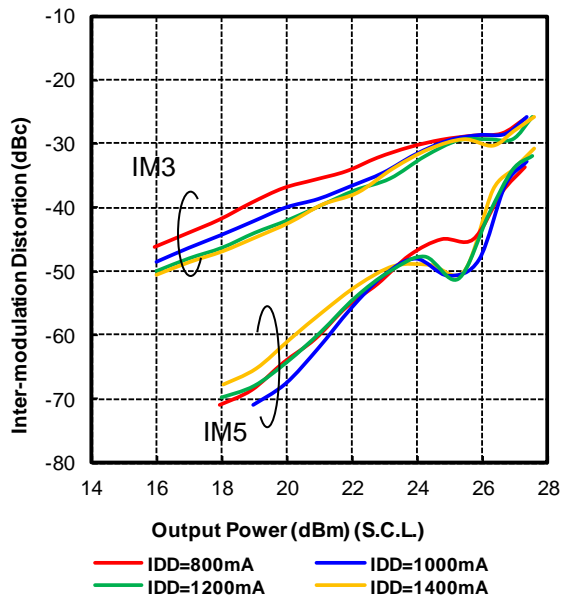
VDD=6V, Freq.=13.5GHz
