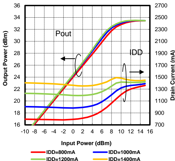
VDD=6V, Freq.=15.4GHz
