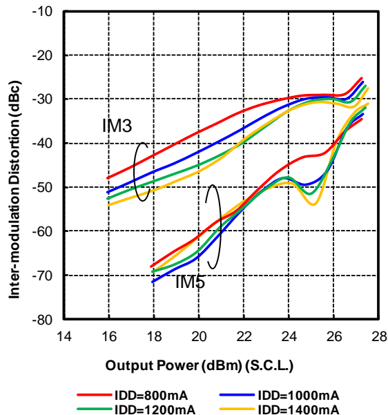
VDD=6V, Freq.=14.5GHz
