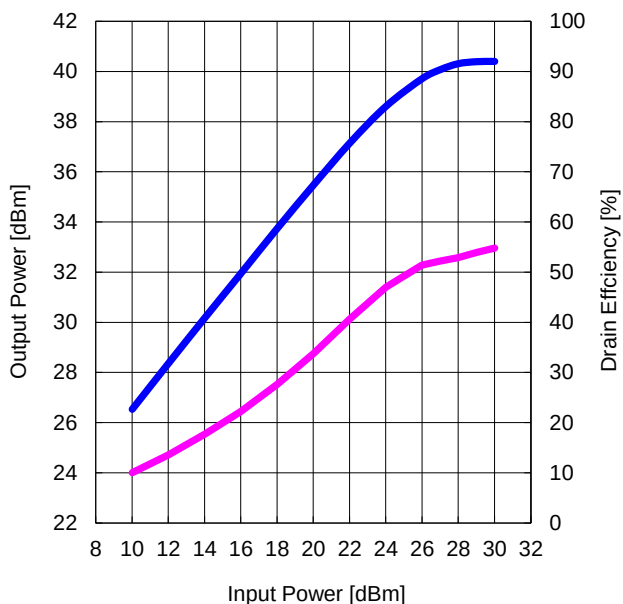
Output Power and Drain Efficiency vs. Input Power V DS =50V I DS(DC) =100mA f=3.5GHz
