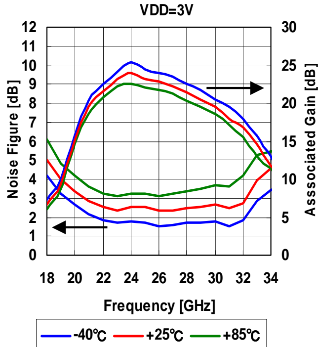
NOISE FIGURE, ASSOCIATED GAIN vs. FREQUENCY by Temperature
