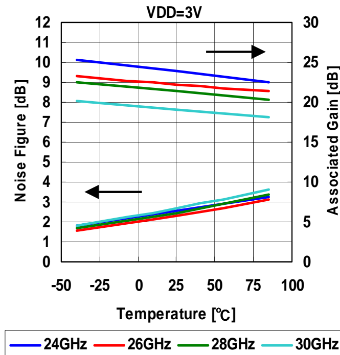
NOISE FIGURE, ASSOCIATED GAIN vs. TEMPERATURE
