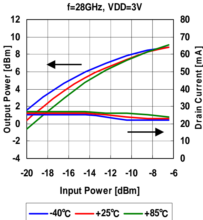
OUTPUT POWER, DRAIN CURRENT vs. INPUT POWER by Temperature
