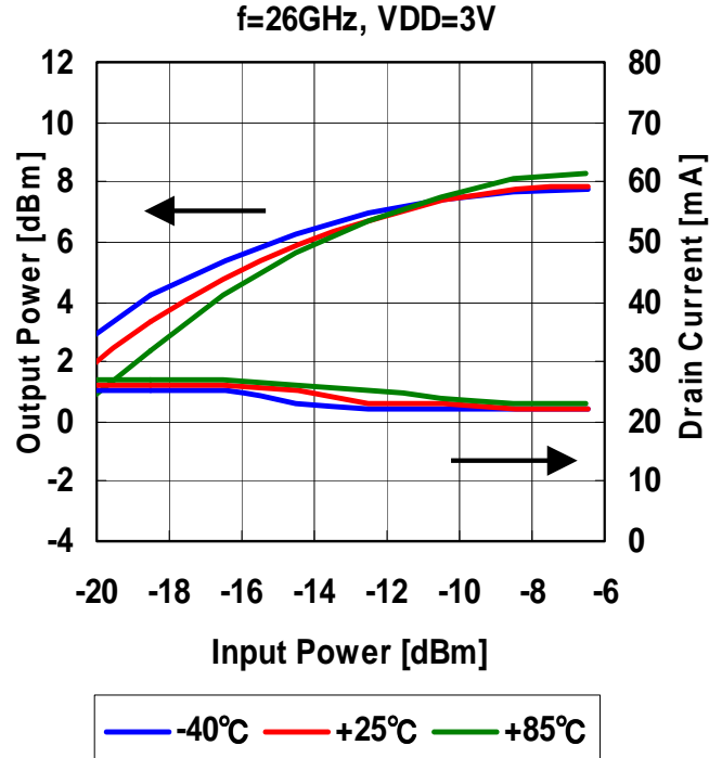
OUTPUT POWER, DRAIN CURRENT vs. INPUT POWER by Temperature
