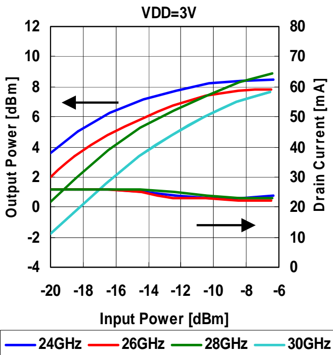
OUTPUT POWER, DRAIN CURRENT vs. INPUT POWER
