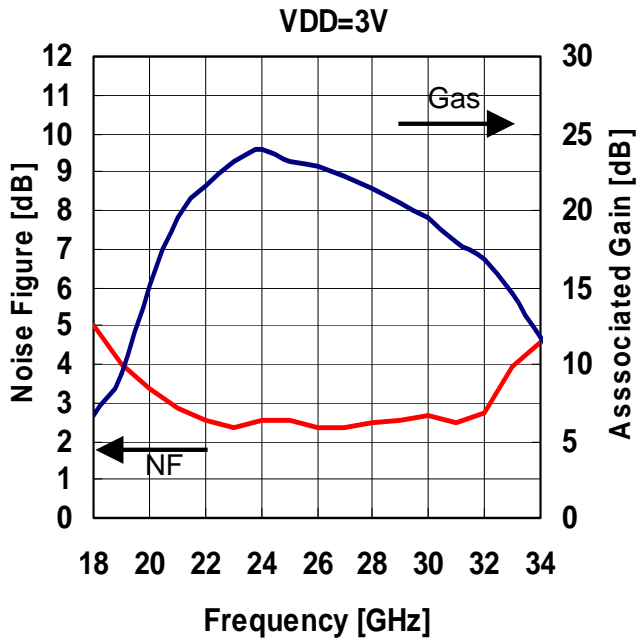
NOISE FIGURE, ASSOCIATED GAIN vs. FREQUENCY
