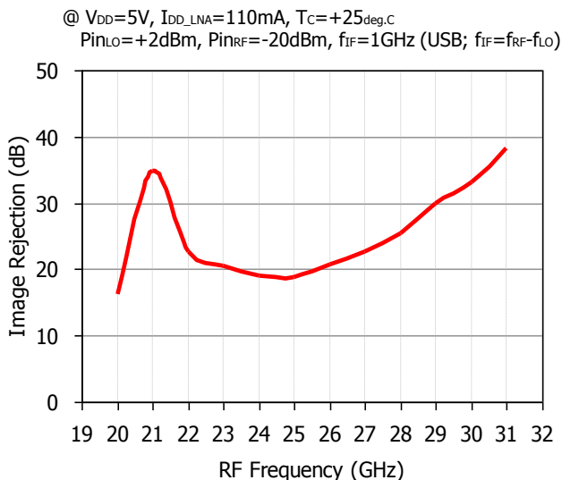
Image Rejection vs. RF Frequency
