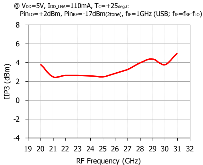
Input IP3 vs. RF Frequency
