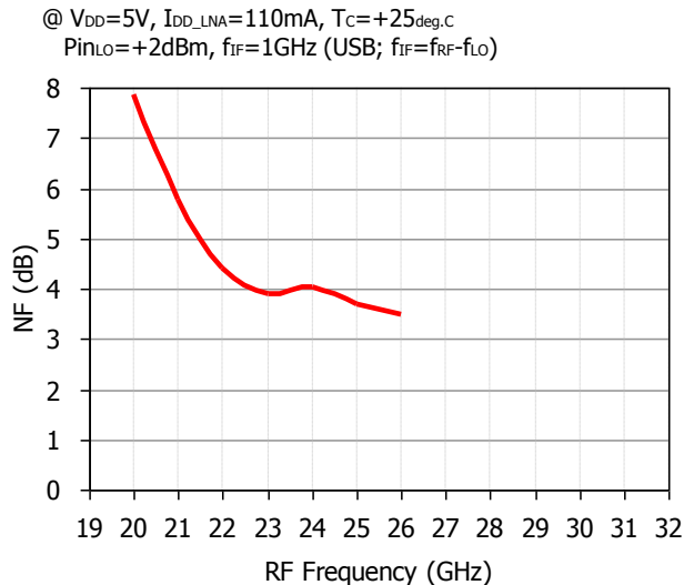
Noise Figure vs. RF Frequency
