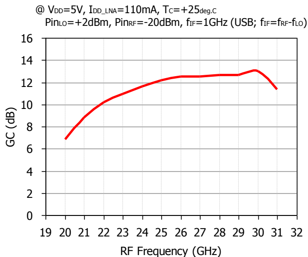
Conversion Gain vs. RF Frequency
