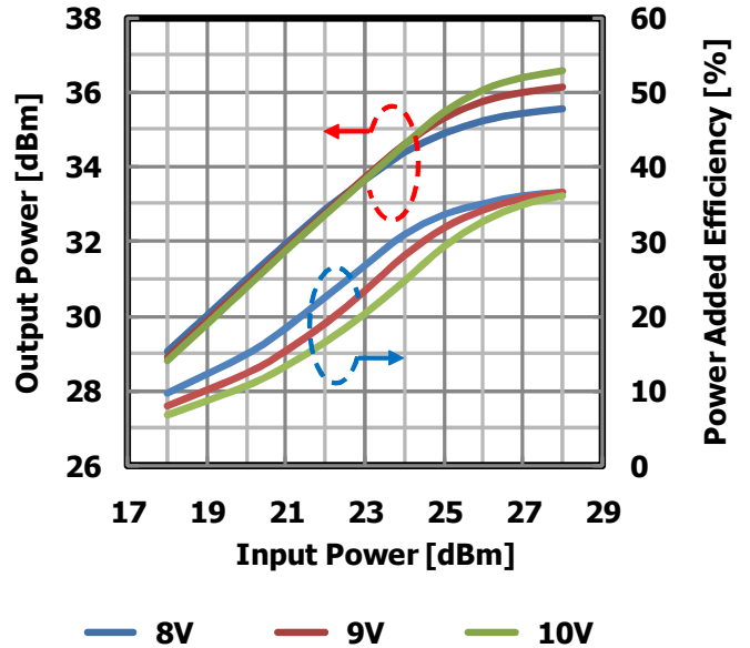
Input Power vs. Output Power, Power Added Efficiency by Drain Voltage I_{DS(DC)} = 1100\text{mA} @7.5GHz
