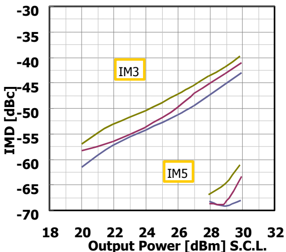
IMD Performance vs. Output Power by Case Temperature V_{DS}=10V I_{DS(DC)}=2200mA @7.2GHz
