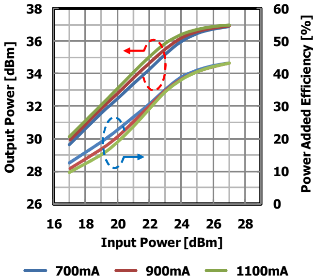
Input Power vs. Output Power, Power Added Efficiency by Quiescent Drain Current V_{DS}=10V @6.4GHz
