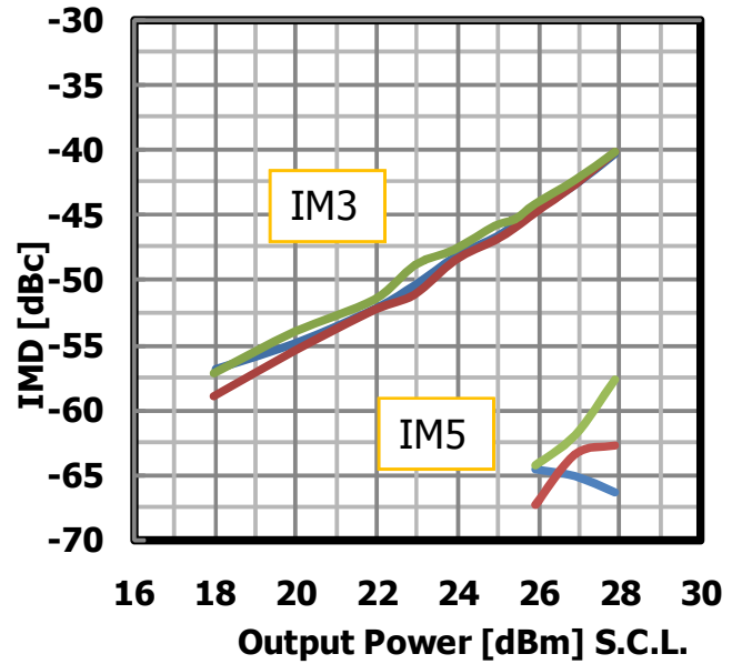
D Performance vs. Output Power by Temperature V_{DS}=10V @6.15GHz
