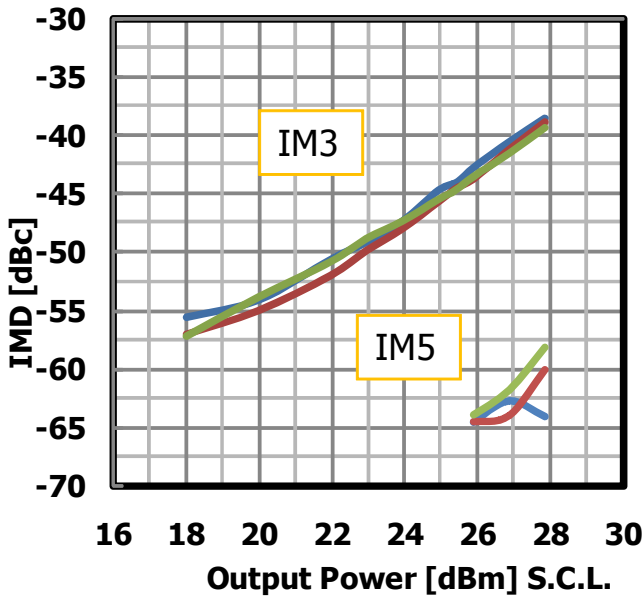
D Performance vs. Output Power by Temperature V_{DS}=10V @5.9GHz
