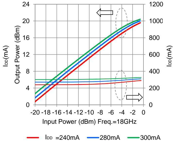
OUTPUT POWER vs. I DD
