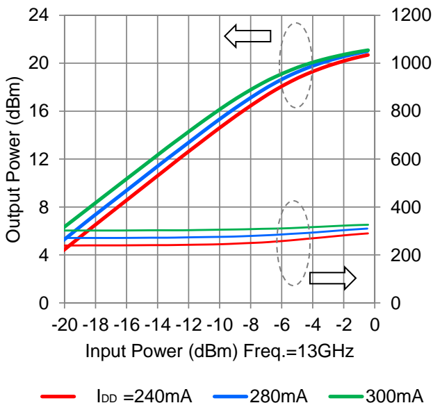
OUTPUT POWER vs. I DD
