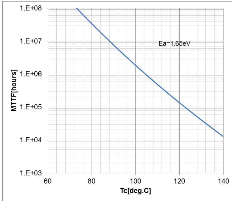
Tc : Temperature at the solder ball Joint
